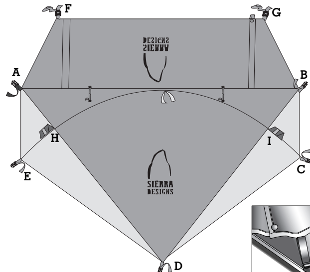
Figure 4: Flysheet (top view)
