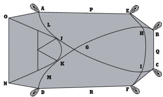
Figure 4: Flysheet (top view)
