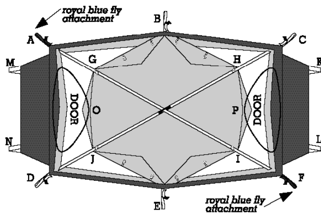
Figure 3: Tent Body (top view)
