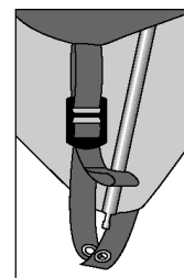
Figure 5: LadderLoc
