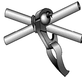
Figure 3: Clip-Loc
