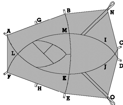
Figure 4: Flysheet (top view)
