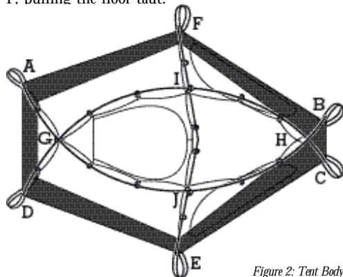
Figure 2: Tent Body (top view)
