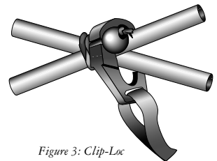
Figure 3: Clip-Loc
